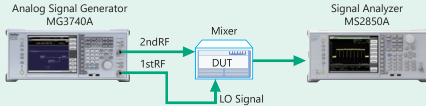
Setup for evaluating distortion characteristics of Mixer
