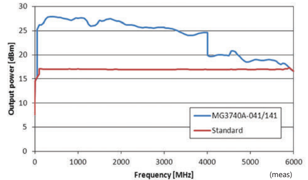
Maximum output power
