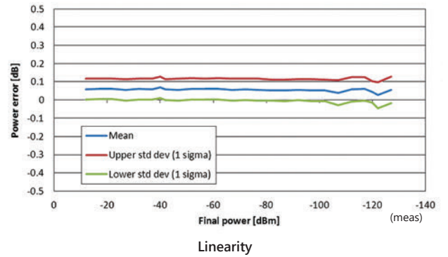
Relative level accuracy at 850 MHz initial power +10 dBm
