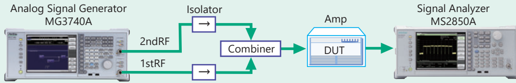
Setup for evaluating intermodulation characteristics of amplifier
