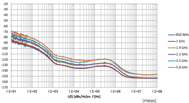
Example: SSB Phase Noise
