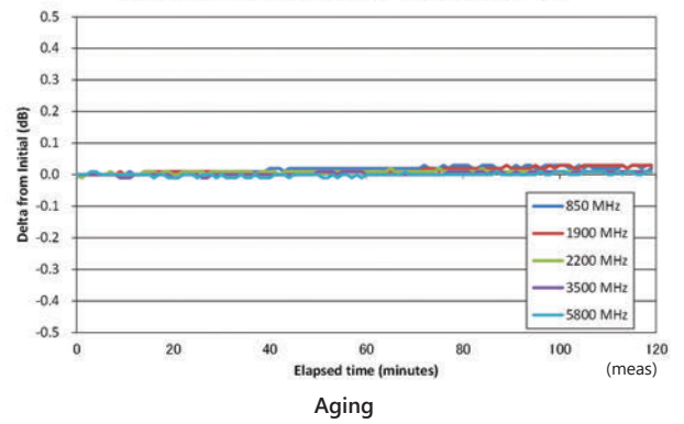
Amplitude repeatability +5 dBm ALC on
