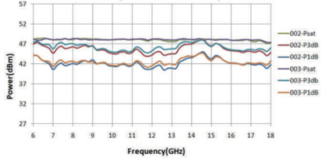
Output Power Vs.Freq.
