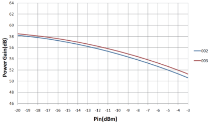
Gain Compression(12GHz)
