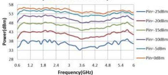
Output Power vs. Freq.
